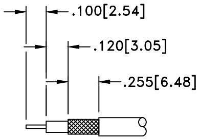
STRIP LENGTHS
