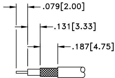
STRIP LENGTHS RG316
